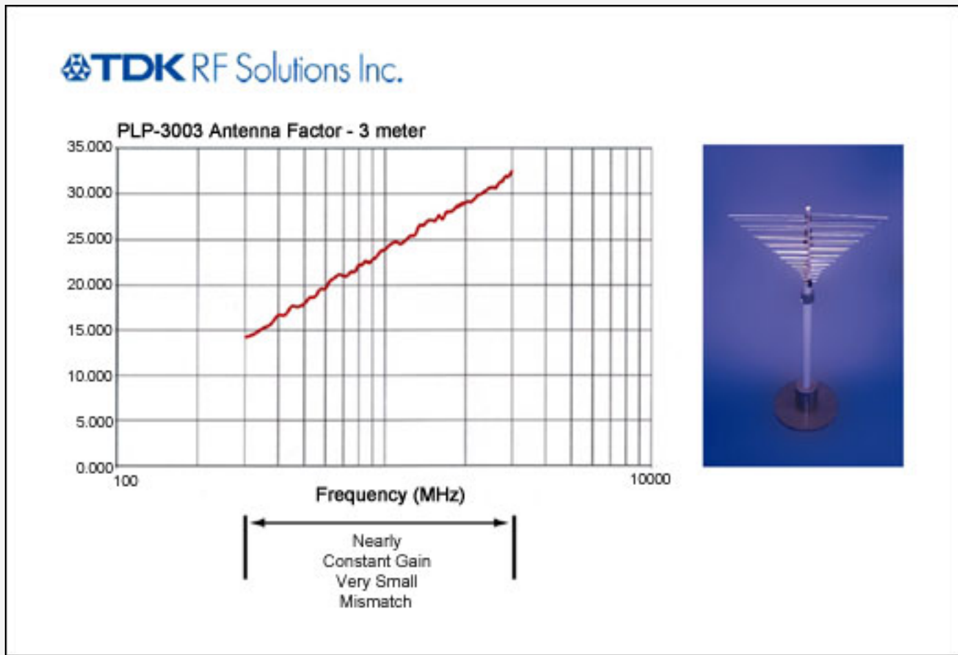
Figure 1. Antenna Factor (AF) vs. frequency of a typical measurement antenna.
