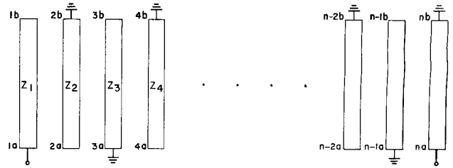
Fig. 2. Schematic interdigital structure showing terminal numbering.
