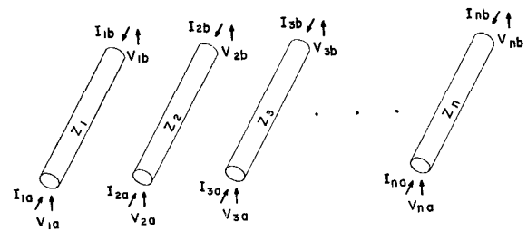
Fig. 1. Schematic array of parallel conductors between ground planes.
