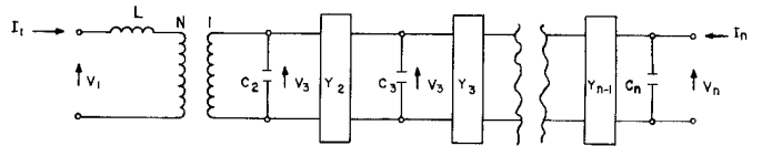
Fig. 3. Equivalent transmission-line cascade.
